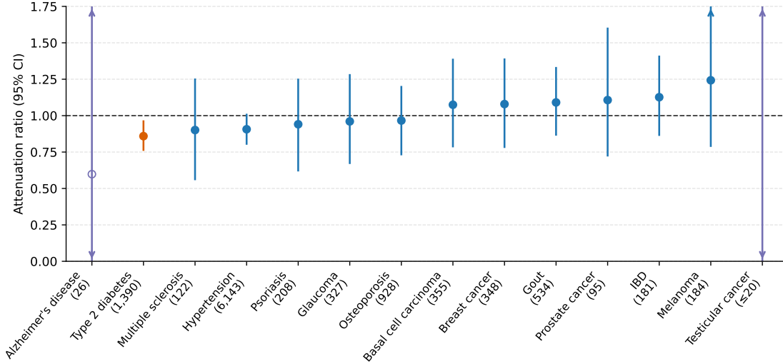
Figure 3: Within-family attenuation ratio across 14 binary traits. Alzheimer’s disease and testicular cancer estimates are unstable due to low case counts. 11 binary traits do not meaningfully attenuate within family, while type 2 diabetes shows slight attenuation in within-family evaluation. Numerical values are provided in Table C3.
