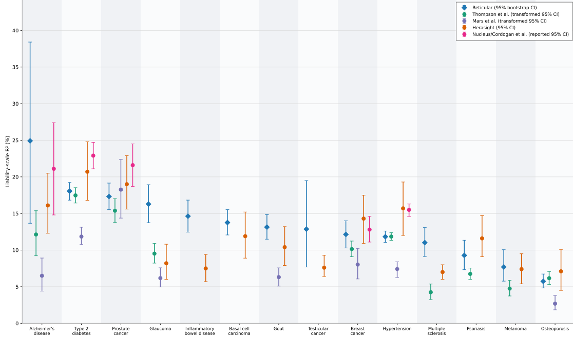
Figure 1: Liability-scale variance explained across 14 binary traits for external-permitted track. Reticular refers to our meta-analysis of external and AoU internal GWAS. We exceed or match the liability variance explained for most traits, though exact phenotype definitions, evaluation cohorts, and populations differ by source. Numerical values provided in Table C1.
